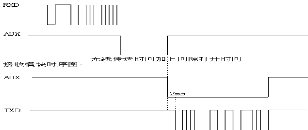
Timing Sequence in Sleep Mode
